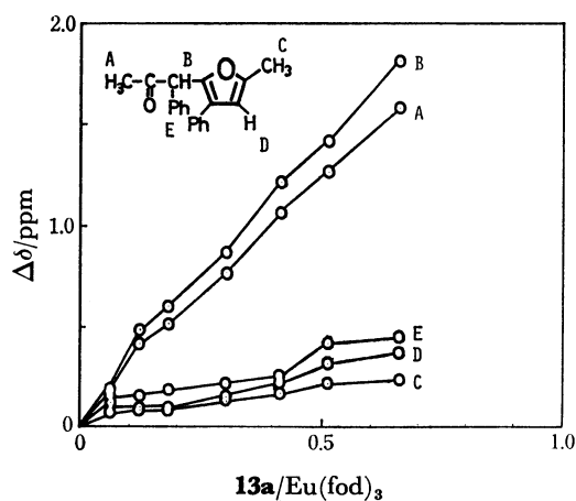
Fig. 4-1. \text{Eu}(\text{fod})_3 -induced shifts for 13a .
